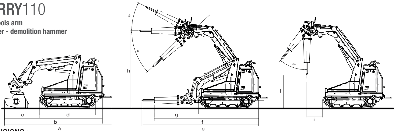
DIMENSIONS (mm)
