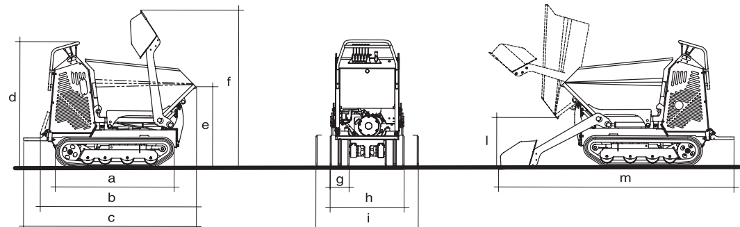
DIMENSIONS (mm)
